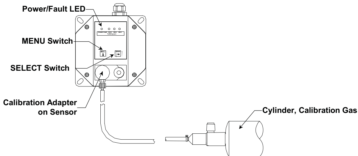
Figure 9: Calibration MRI-5175
